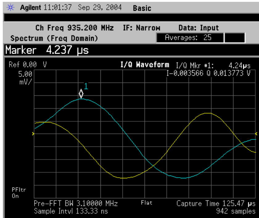
Figure 2-3 Spectrum (Time Domain) Measurement - I/Q Waveform Result (PSA Series View)
