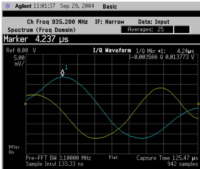
Figure 3-2 Spectrum (Time Domain) Measurement - I/Q Waveform Result
